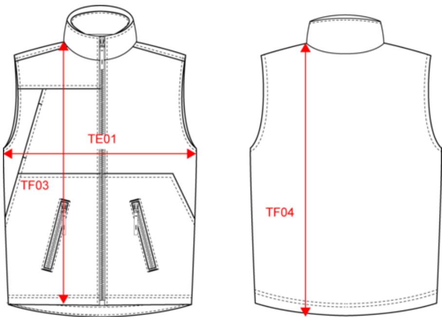
Dimensions (cm)
